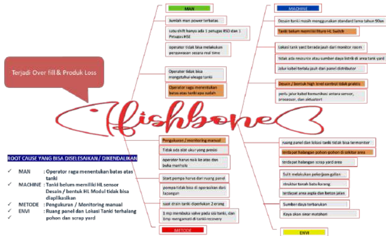
Gambar 2. Fishbone Diagram
