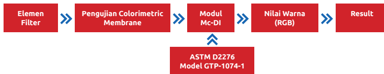
Gambar 3. Block Diagram Cara Kerja MCDI
