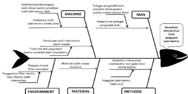
Gambar 2. Fishbone Diagram
