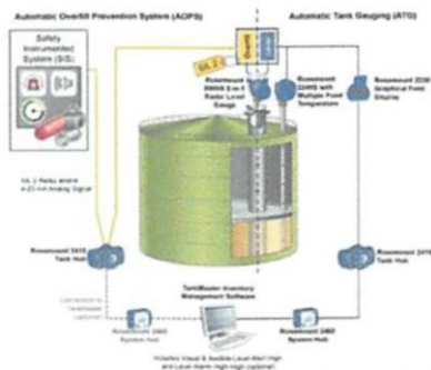
Gambar 2.1 Oil Level Reader
